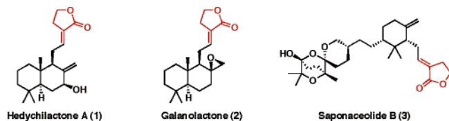
Figure 1. Natural products bearing the \alpha -alkylidene- \gamma -butyrolactone substructure.
